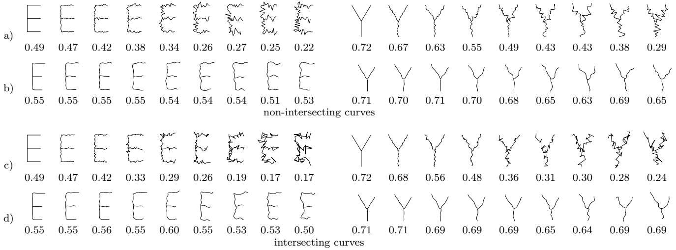
Fig. 5 a) & c) increasing amounts of noise are added to two letters; b) & d) the noise is reduced by smoothing. Values of \mathcal{L}_{comp}(C) are provided to show the effects of noise and smoothing.
