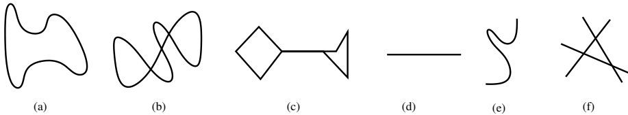
Fig. 2 Several curve examples which will be treated here as closed curves are in (a)-(e). An example of connected compound curve is in (f).
