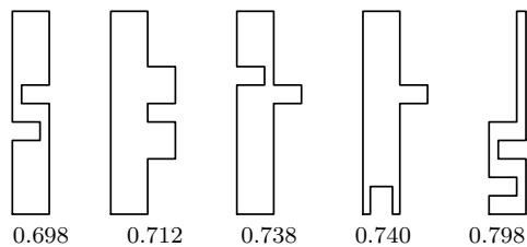
Fig. 1 The value of \mathcal{I}_{closed}(\mathcal{C}) is 0.699 for all the shapes, but the proposed measure \mathcal{L}_{cl}(\mathcal{C}) produces different linearities (shown below).
