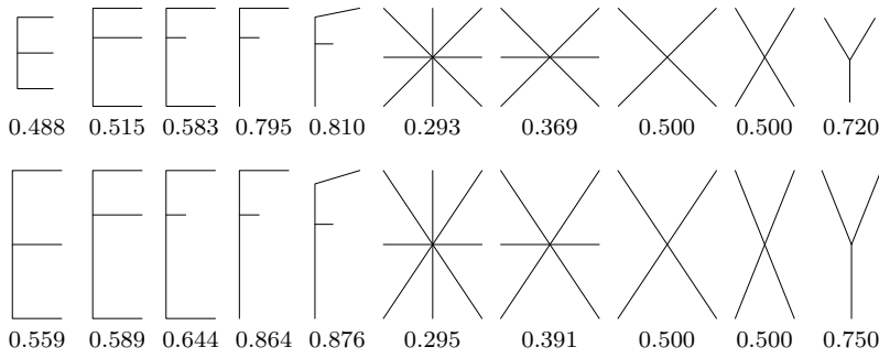
Fig. 4 Values of \mathcal{L}_{comp}(C) for synthetic curves containing multiple components.
