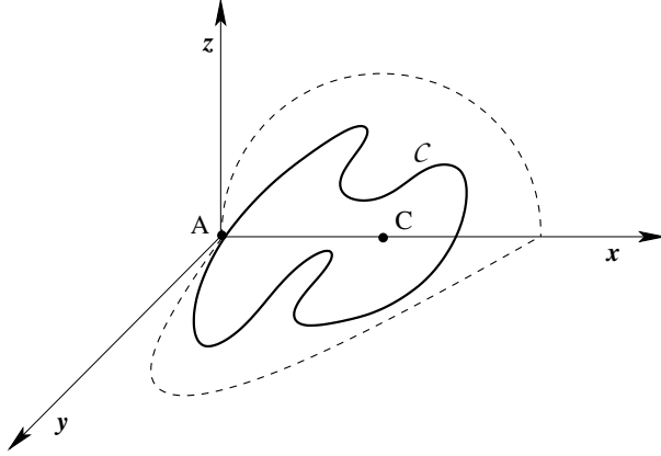
Fig. 3 A is a point from the curve C which is furthest from the curve centroid C .
