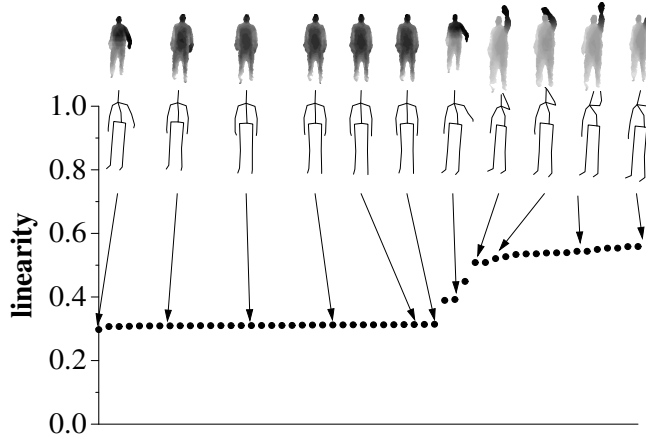
Fig. 6 2D views of 3D skeletons extracted from depth maps taken from an action sequence and plotted with their \mathcal{L}_{comp}(\mathcal{C}) values.
