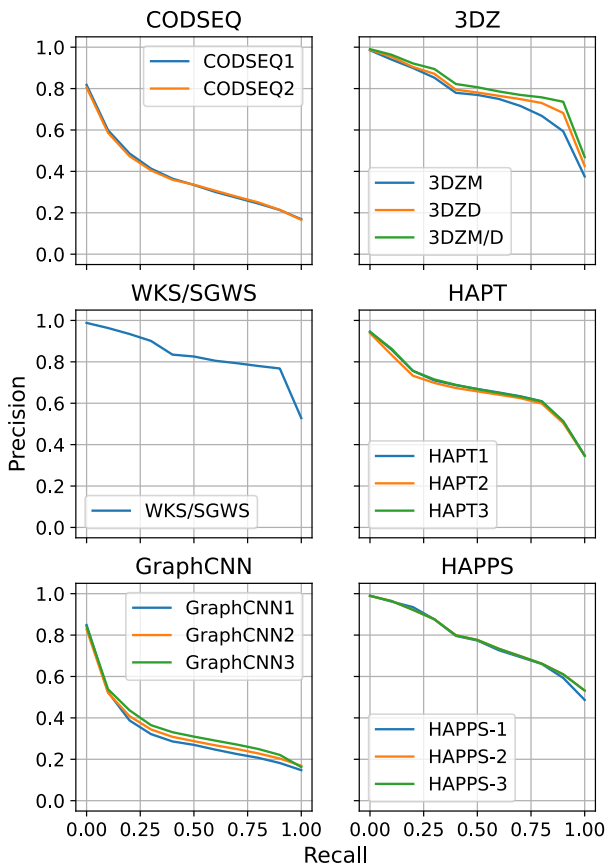
Fig. 4. Precision-Recall curves at the protein level.
