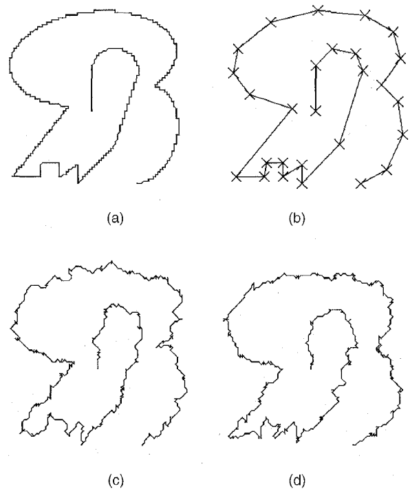
Fig. 10. Examples of curves used for evaluating metrics. (a) Uncorrupted test curve. (b) Model segmentation using E_{\infty} metric. (c) and (d) Test curve with noise.
