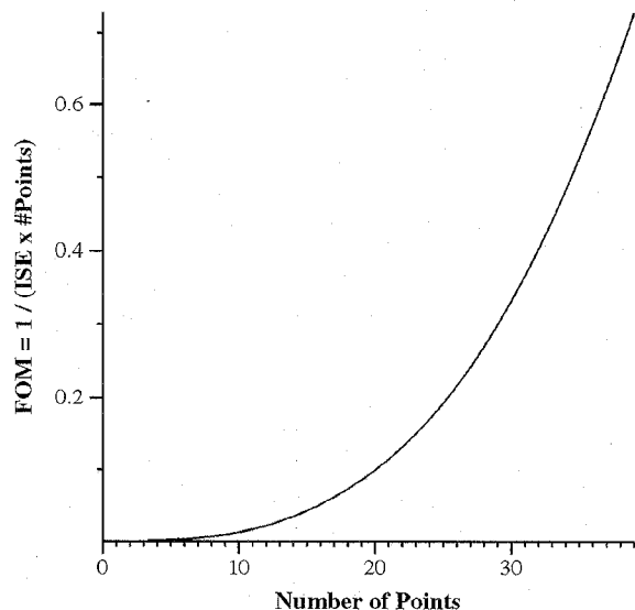
Fig. 1. Theoretical FOM of optimal polygonal approximation for a circle ( r=10 ).
