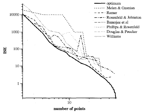
Fig. 7. ISE curves of optimal and other algorithms.
