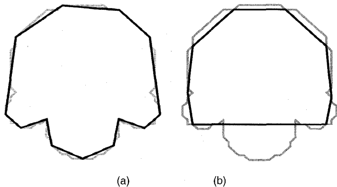
Fig. 6. Some approximations of Fig. 4. (a) Result of Lowe's algorithm. (b) Result of Sankar and Sharma's algorithm.
