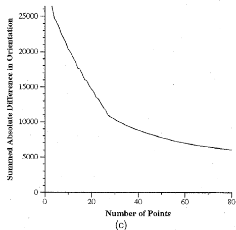
Fig. 2. Effects of natural scales on approximation error. (a) Circle with superimposed sine wave. (b) ISE of optimal polygonal approximation. (c) SADO of optimal polygonal approximation.
