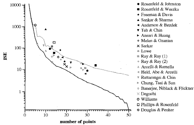
Fig. 5. ISE of optimal and other algorithms.
