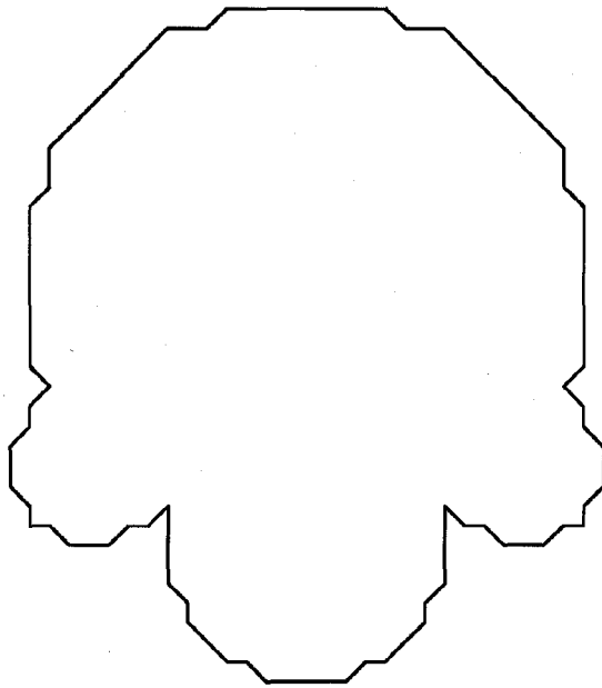
Fig. 4. Curve used by Teh and Chin.
