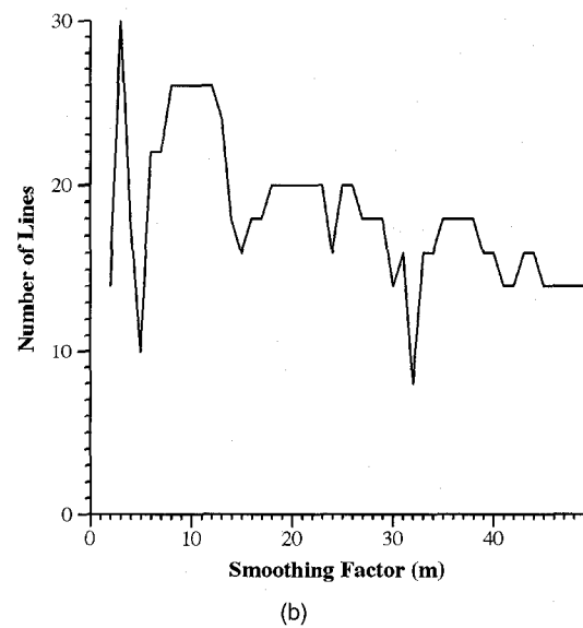
Fig. 8. Effect of smoothing parameter on the detected number of dominant points. (a) Rosenfeld and Johnston's algorithm. (b) Phillips and Rosenfeld's algorithm.
