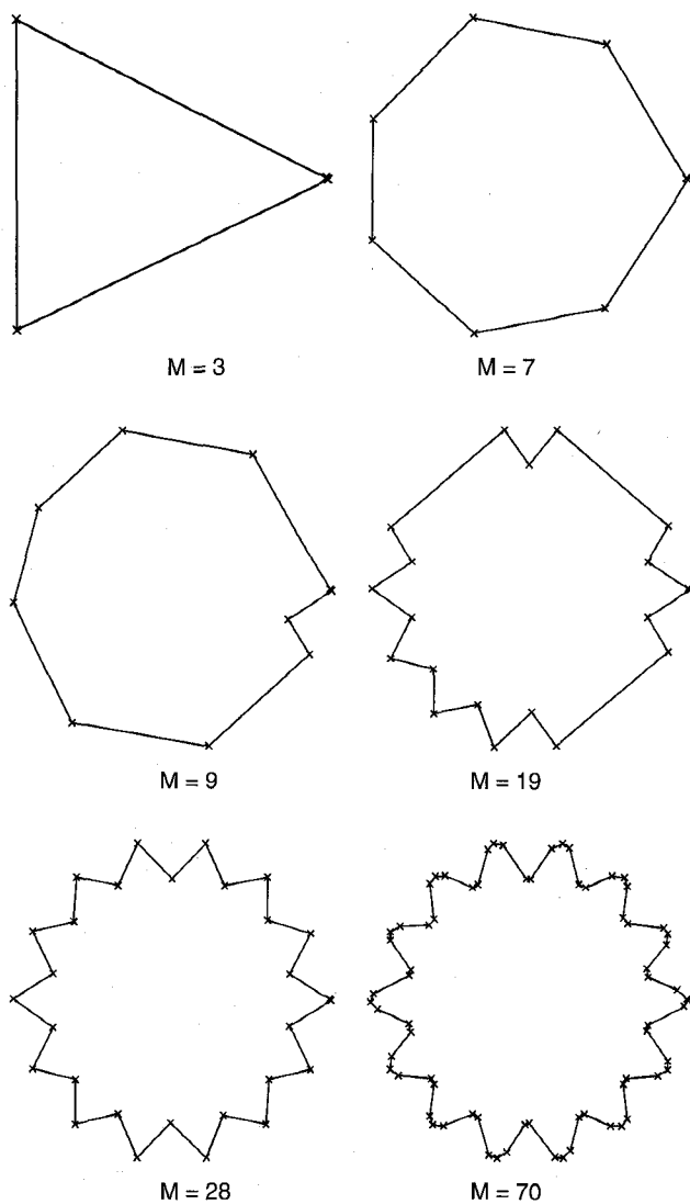
Fig. 3. Effects of natural scales on the shape of the approximations.
