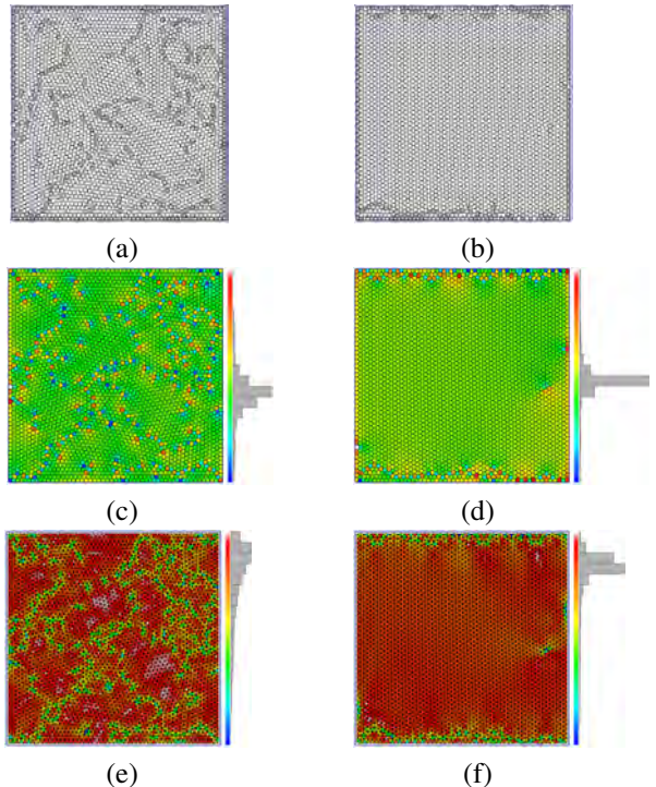
Figure 4: Two CVTs with 3,000 seeds in a square. Left column: random initialisation, converging to an energy of 6.47582 \times 10^{-4} ; right column: Hammersley initialisation, converging to an energy of 6.46110 \times 10^{-4} .
