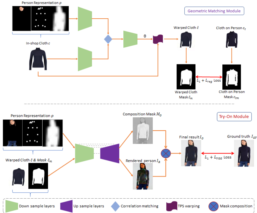
Figure 2. Full pipeline of our proposed CP-VTON+.
