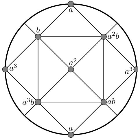
Figure 12: A projective embedding of \overline{\mathcal{P}^*(D_8)} . (corrected)
