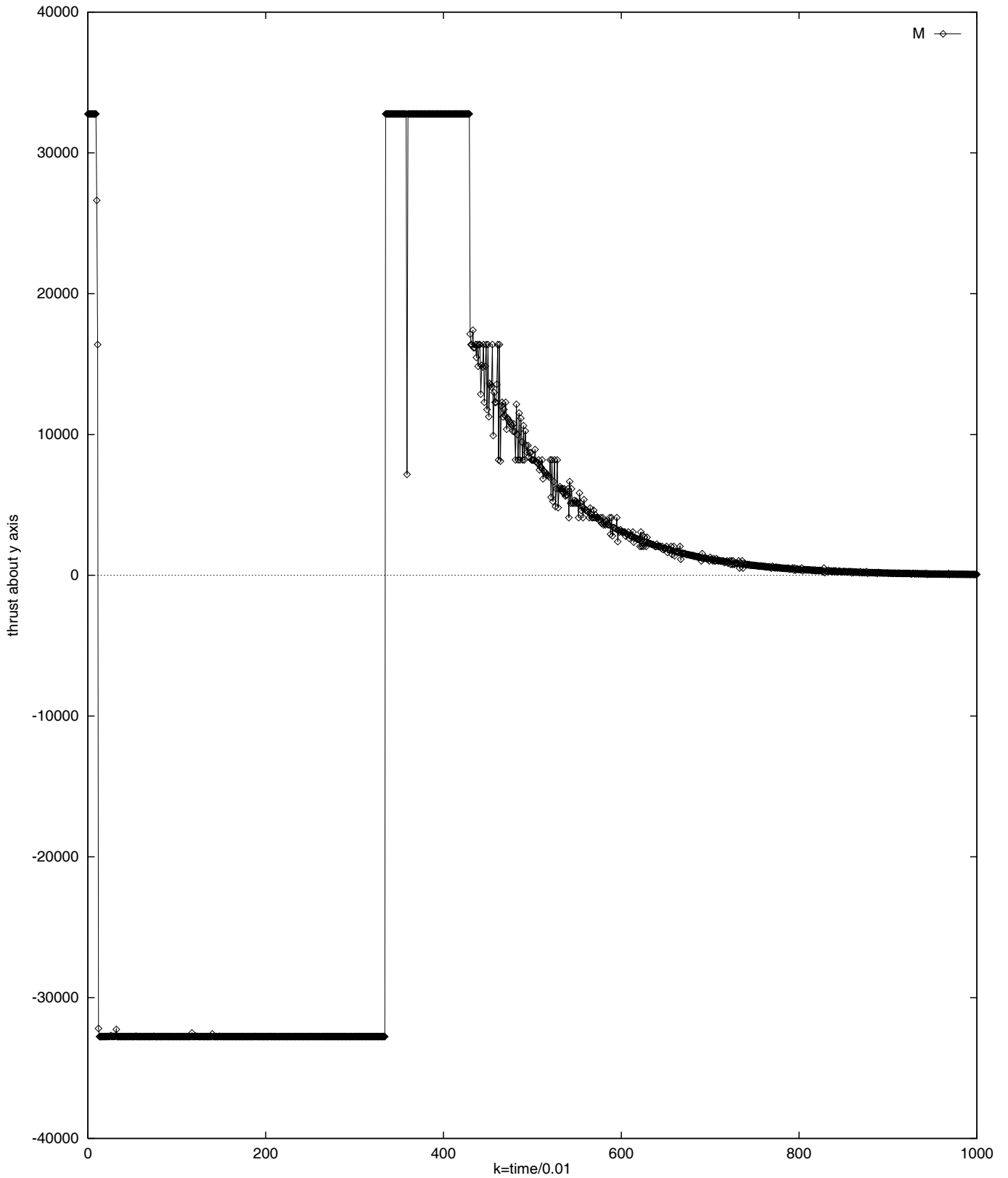
Fig. 14. Applied thrust G_2 about the y body axis for the satellite, in the presence of forces trying to lead it in a chaotic motion, during the application of the Neuro-Genetic Controller. Initial conditions (\omega_1, \omega_2, \omega_3) = (2.0, 1.5, 1.7) and (\phi, \theta, \psi) = (2.2, 2.2, 2.2) .
