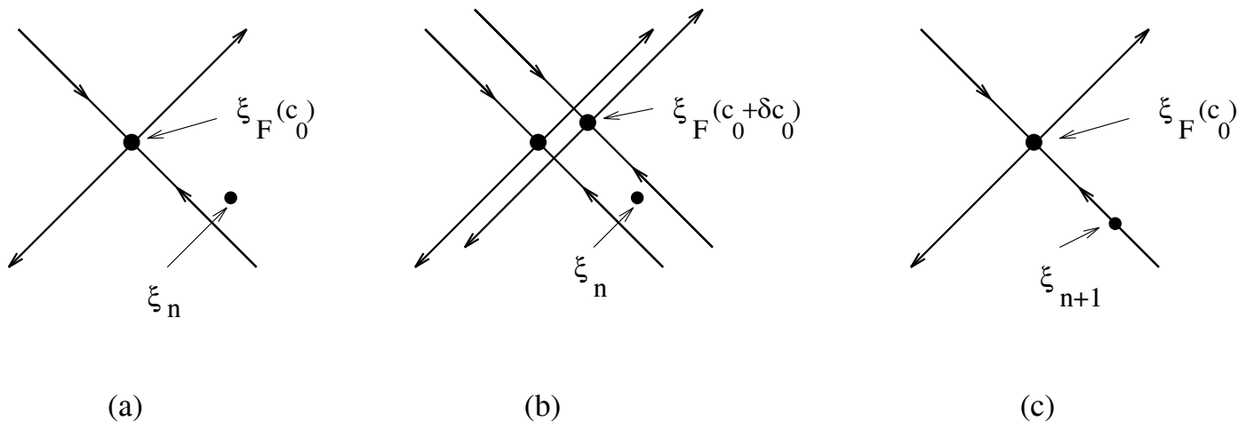
Fig. 5. An example of the OGY method application.
