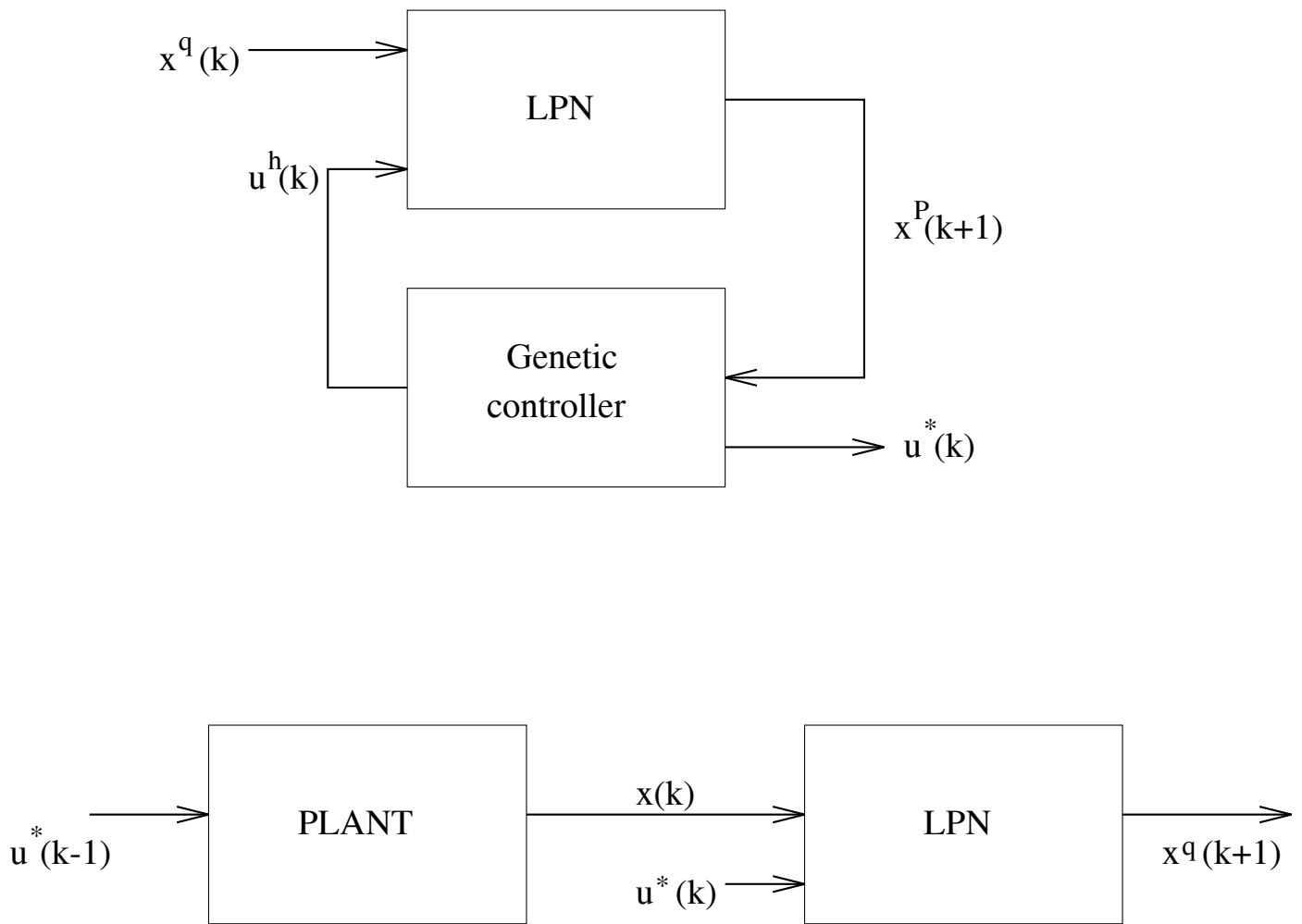
Fig. 4. The adaptive neuro-genetic architecture.
