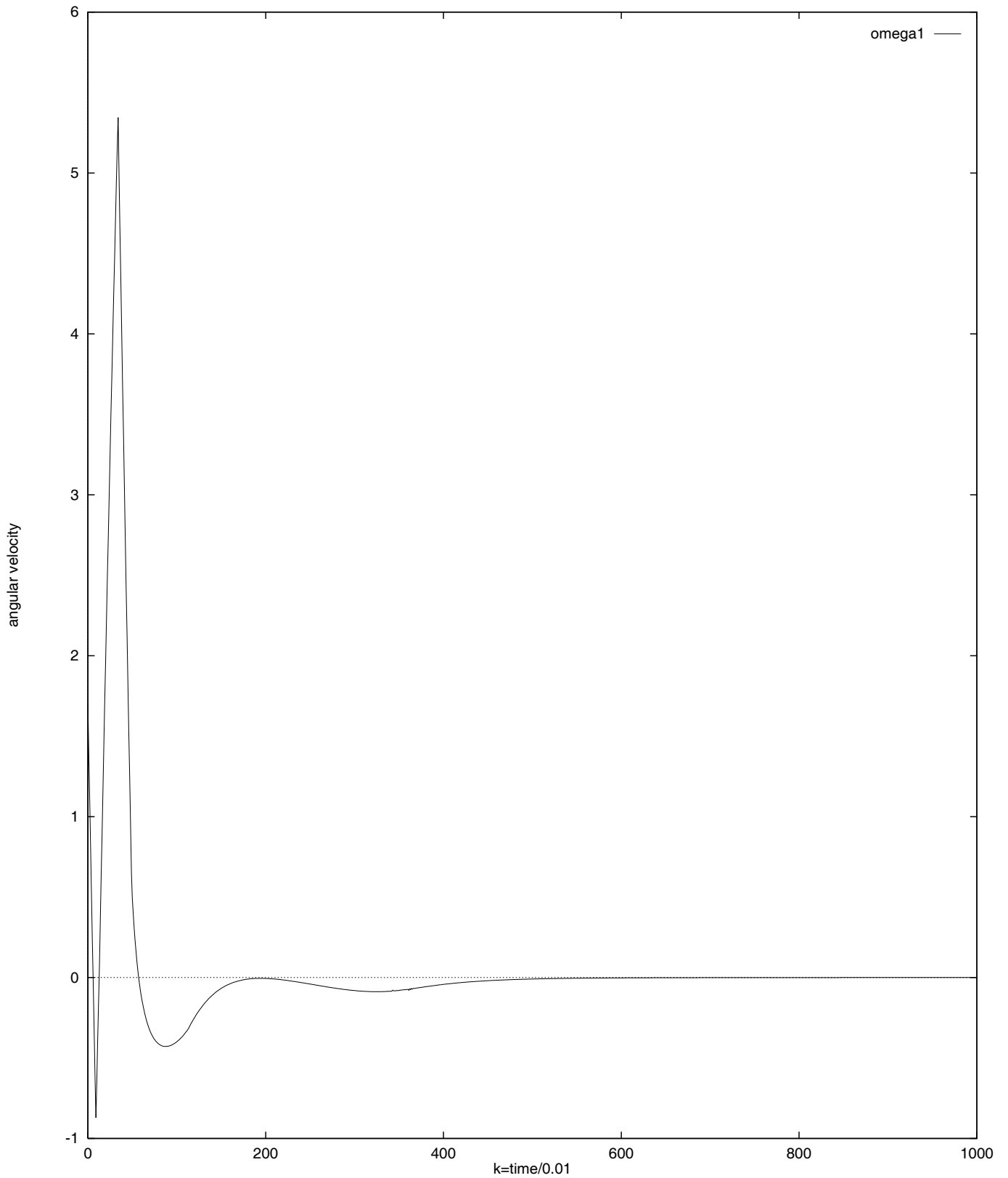
Fig. 7. Angular velocity \omega_1 for the satellite, in the presence of forces trying to lead it in a chaotic motion, after the application of the Neuro-Genetic Controller. Initial conditions (\omega_1, \omega_2, \omega_3) = (2.0, 1.5, 1.7) and (\phi, \theta, \psi) = (2.2, 2.2, 2.2) .
